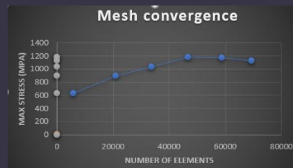
Mesh Convergence Curve
