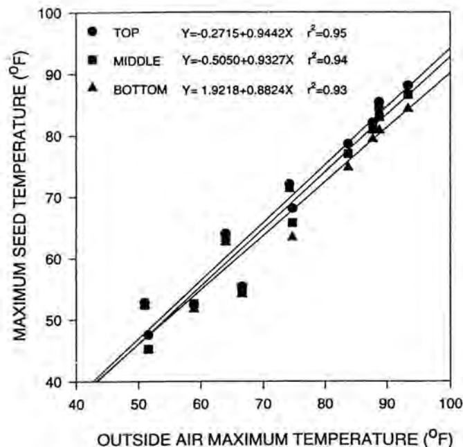
Figure 5. Relationship between ambient outside maximum temperature and maximum seed temperature at different locations (top, middle, and bottom) in stacks in open storage. Y = maximum seed temperature (°F); X = maximum outside temperature (°F).
