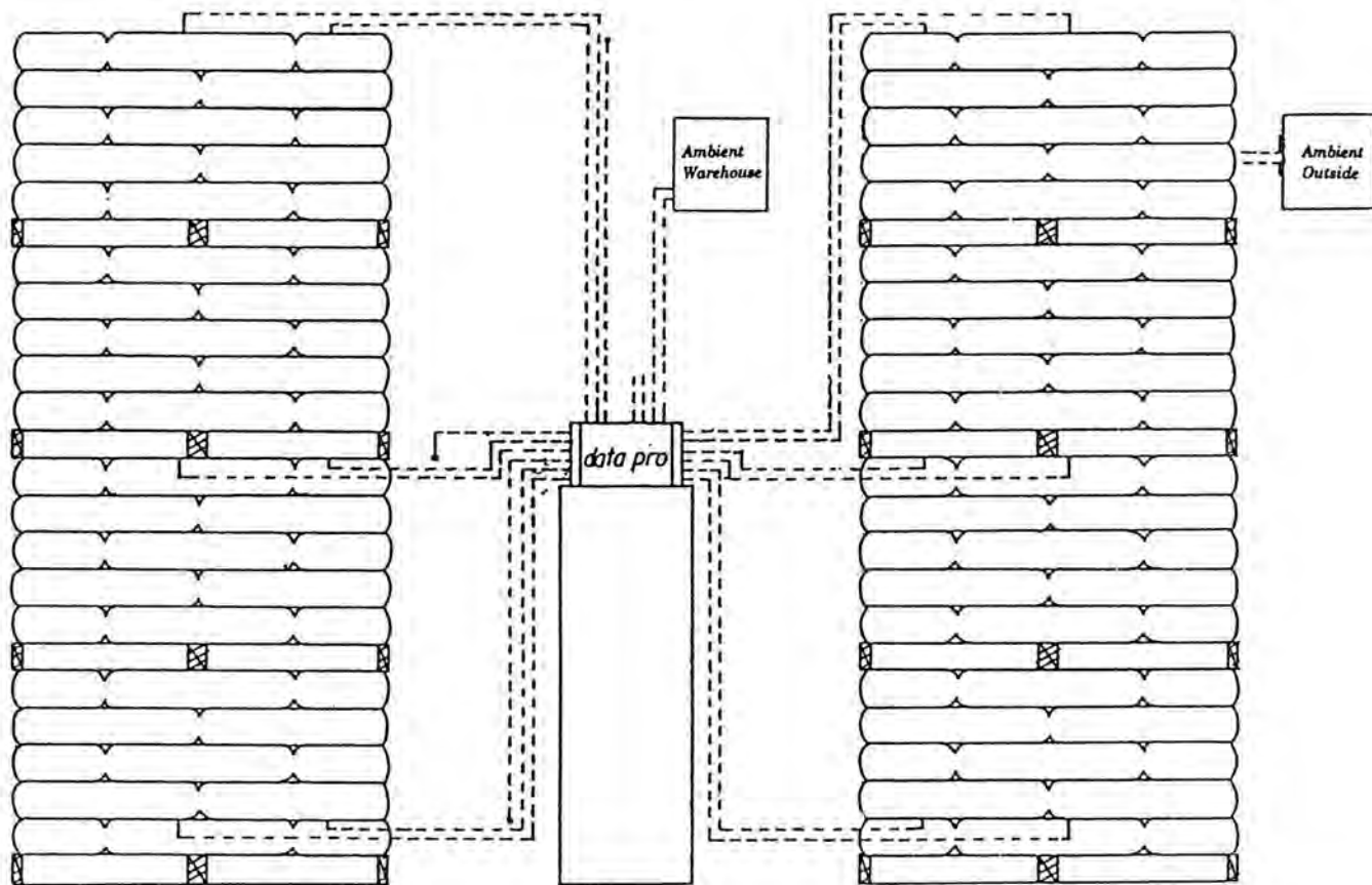
Figure 1. Seed stack arrangement and location of thermocouples in two stacks of soybean seed. Each stack consists of 160 bags comprised of four pallets, each containing 40 bags in five layers of eight bags each. The term “location” refers to the placement of thermocouples in the bottom, middle, and top of the stack. The term “position” indicates the placement of the thermocouples in an outer or inner bag with respect to the stack.
