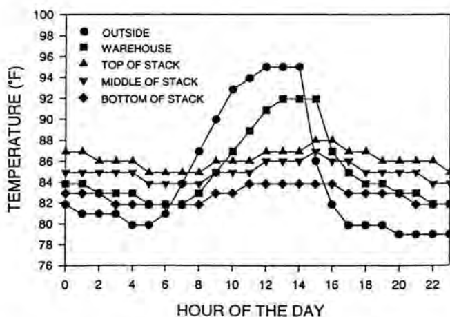
Figure 10. Hourly ambient outside air, ambient warehouse, and seed temperatures at three locations (top, middle, and bottom) with respect to height in stack in an open storage warehouse on July 15, 1986.
