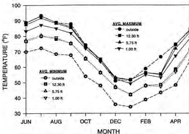
Figure 3. Average monthly maximum and minimum ambient outside temperatures and monthly maximum and minimum ambient temperatures measured at different heights inside an open warehouse.
