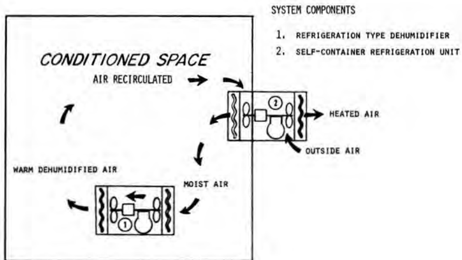
DEHUMIDIFICATION AND COOLING SYSTEM, TYPE VI
