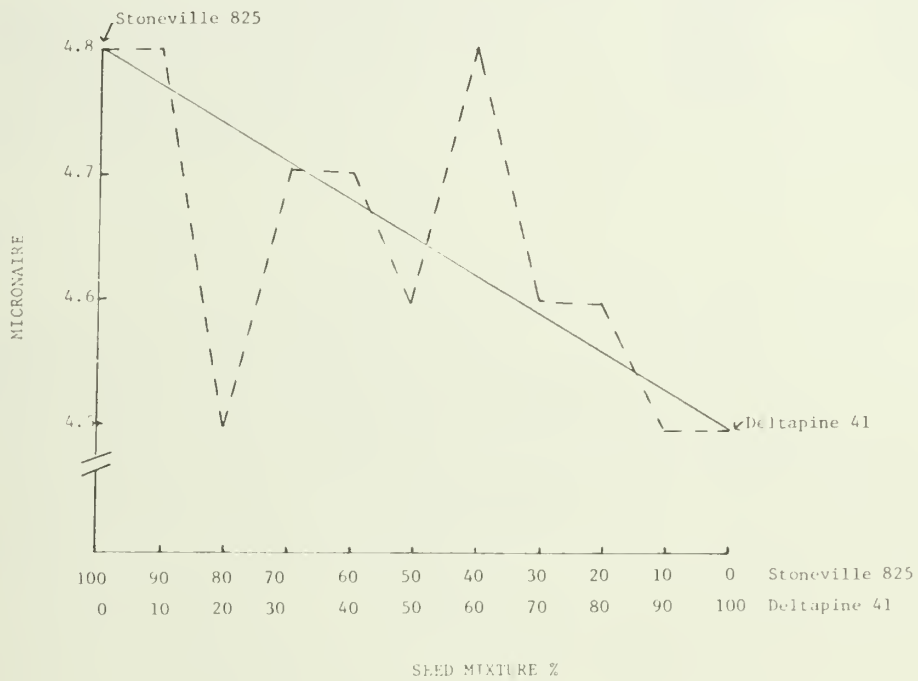
Figure 6. Influence of seed mixtures on micronaire.
