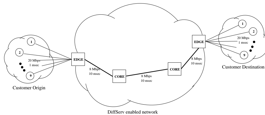
Figure 4.1 Simulation Topology
