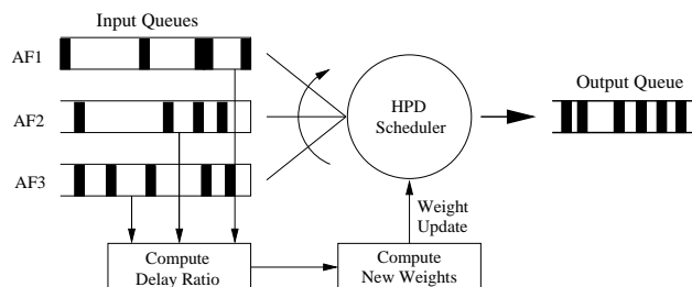
Figure 3.1 Adaptive HPD
