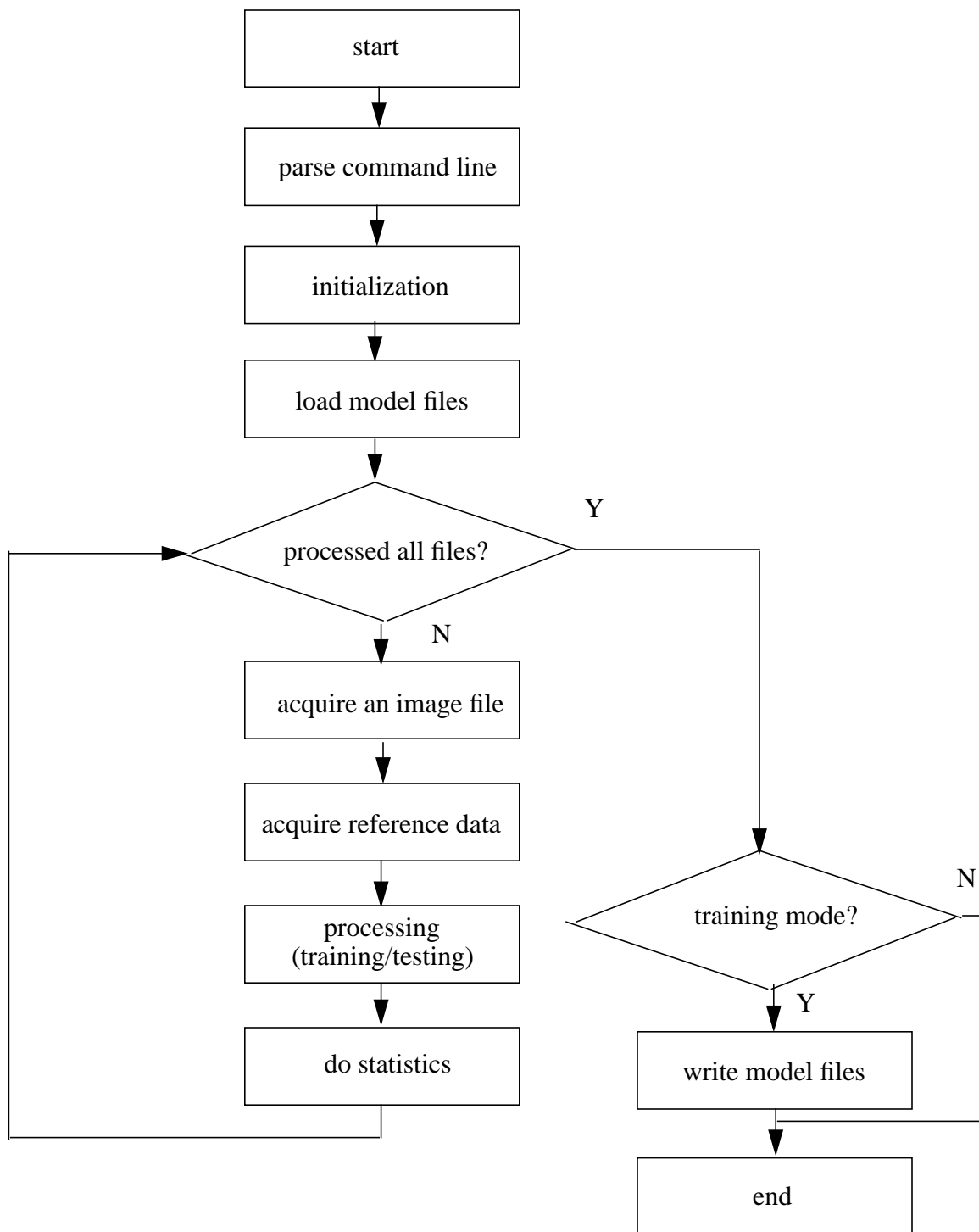
Figure 18. The flow chart for the shell program of the segment_image utility.
