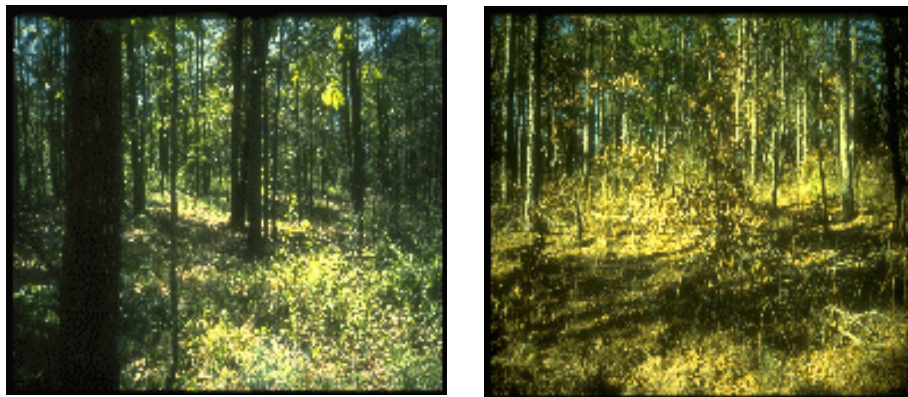
Fractal Dimension = 2.32, SBE = 31.20 Fractal Dimension = 0.14, SBE = -85.57
